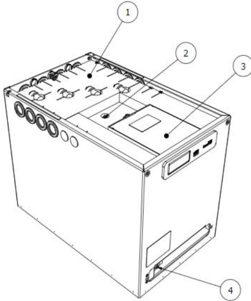
Figure 2: Heat Battery (internal)
